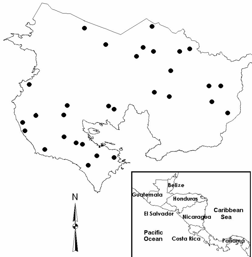
Figure 1. Location of the plantations sampled in northern Costa Rica
