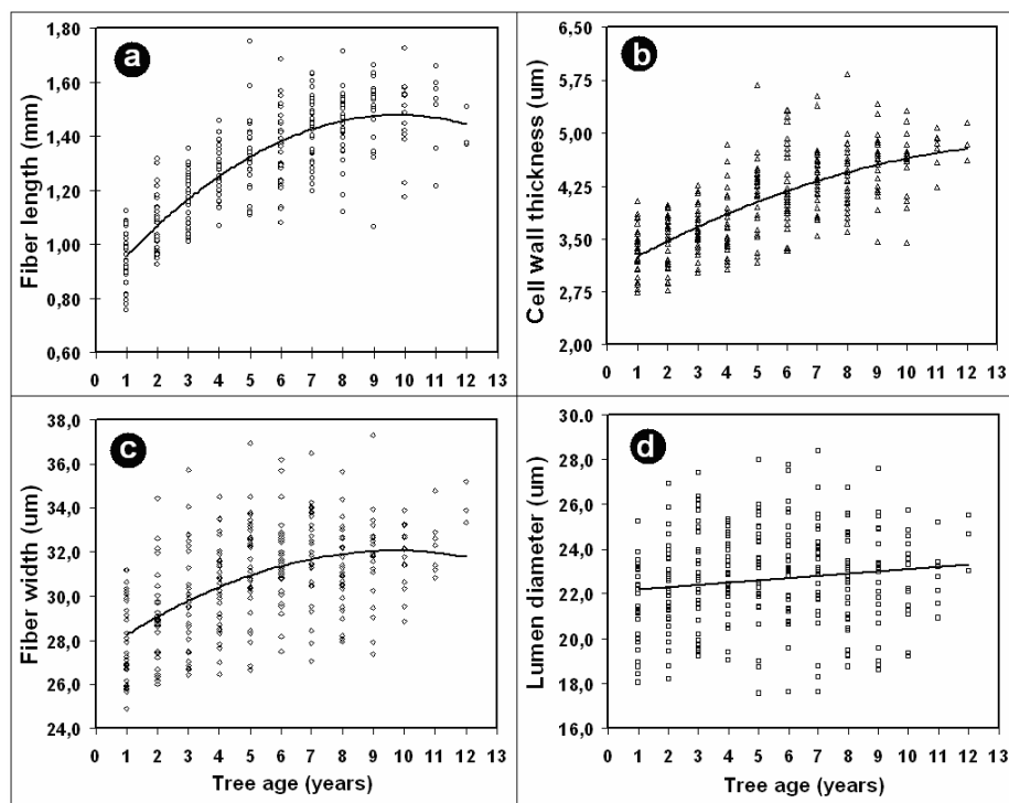
Figure 4. Variation in the fiber dimension of Gmelina arborea from a fast growth plantation in Costa Rica
