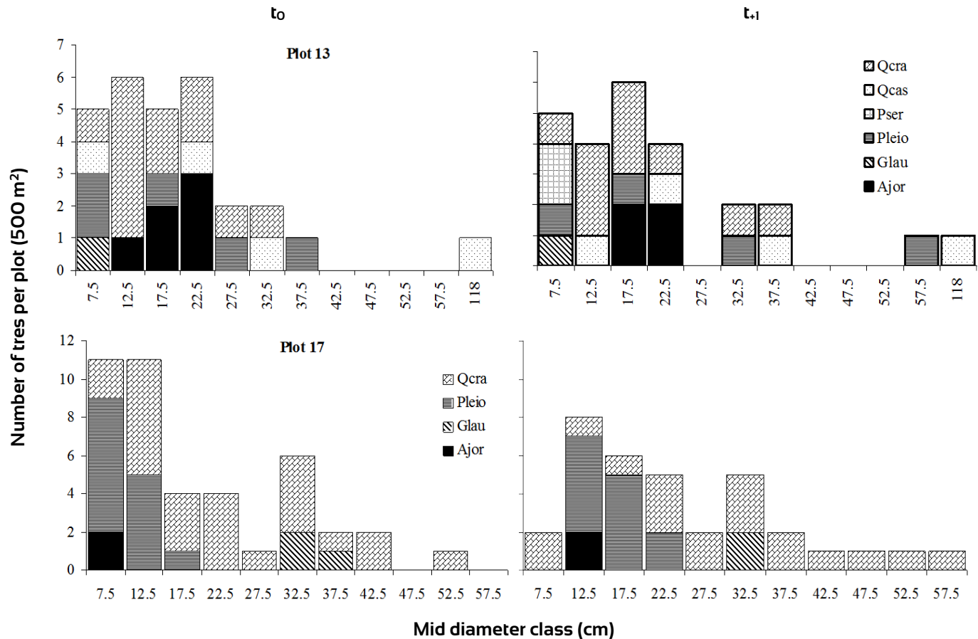
FIGURE 3. Diameter class distributions of plots with different rates of change based on I p dynamics in xeric zone. Ajor, Alnus jorullensis ; Glau, Garrya laurifolia ; Pleio, Pinus leiophylla ; Pser, Prunus serotina ; Qcas, Q. castanea ; Qcra, Q. crassipes .
